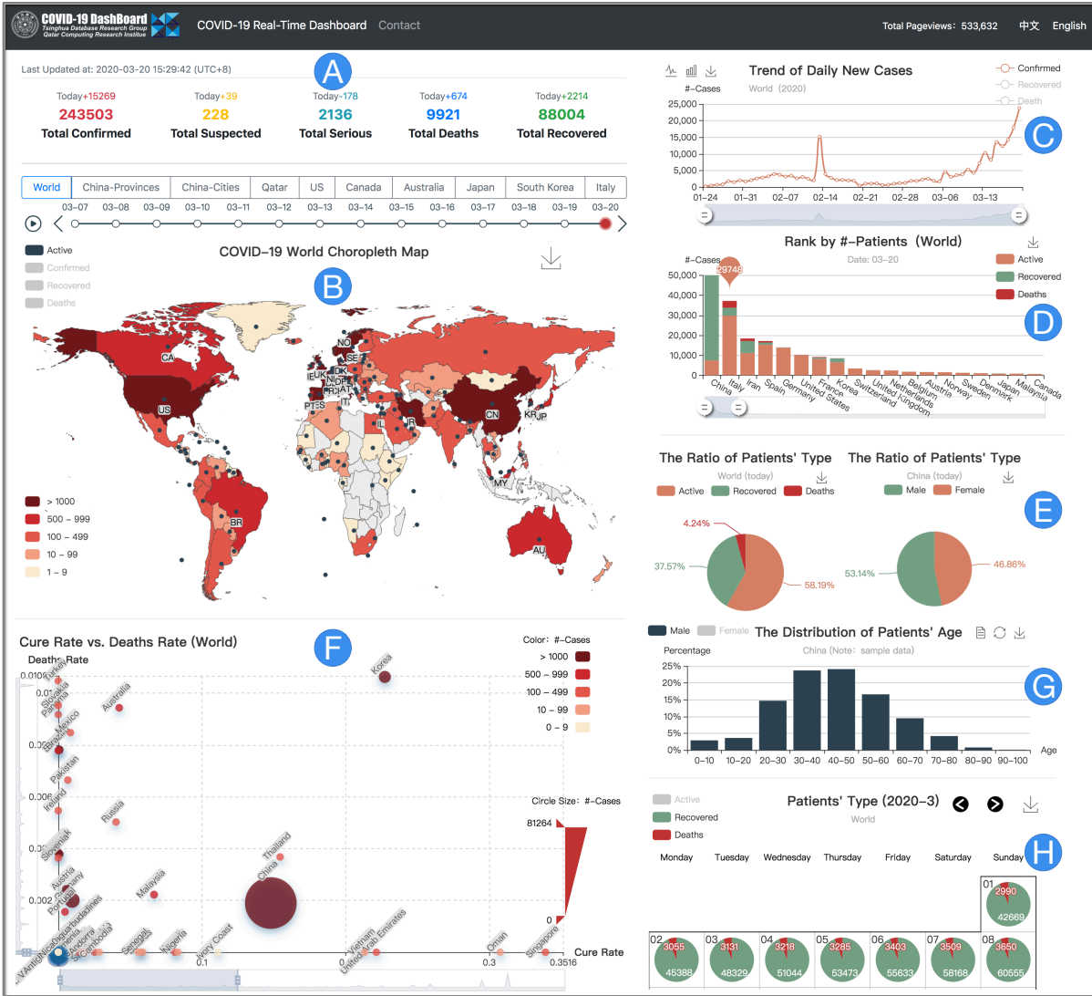
Figure 2: Demonstration of DEEPTRACK-COVID-19 ( https://ncov.deepeye.tech/en )
