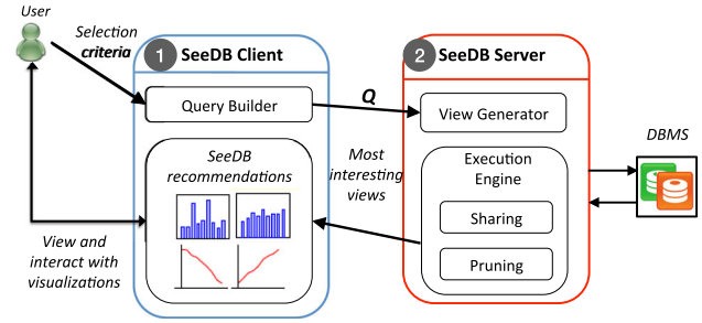
Fig. 12 The architecture of SeeDB [22]. Client (①) accepts users' input, constructs visualization queries and shows recommended visualizations to users. Server (②) generates visualization candidates (view generator) and recommends visualizations to users (execution engine)
