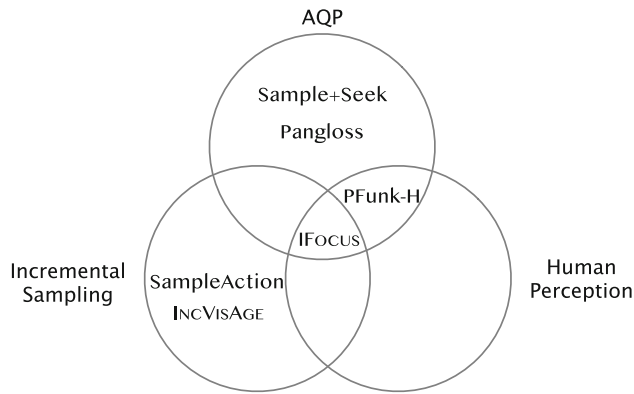
Fig. 7 A classification of approximate data visualization, where the surveyed works are classified as AQP, incremental sampling, and human perception methods
