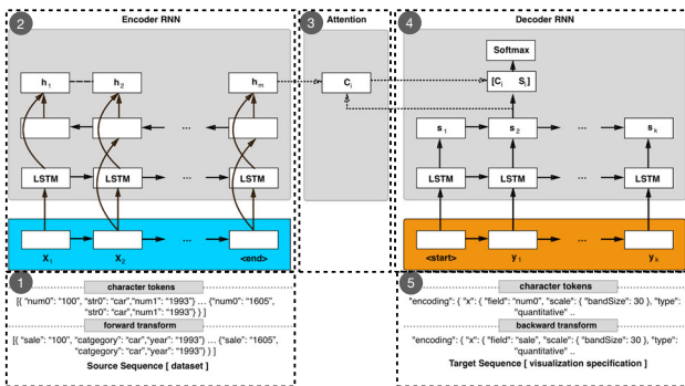
Fig. 11 The architecture of Data2Vis [120]. Data2Vis is built based on sequence to sequence model with the encoder–decoder architecture (② and ④) and the attention mechanism (③). It takes original datasets (①) as input and automatically recommends visualizations (⑤) by given datasets (①)
